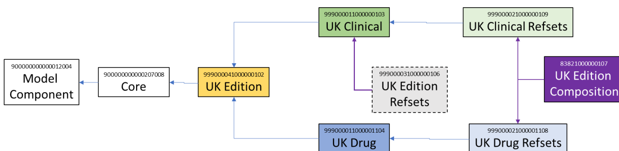
Figure 2: UK Edition Module Dependency Tree from June 2019
